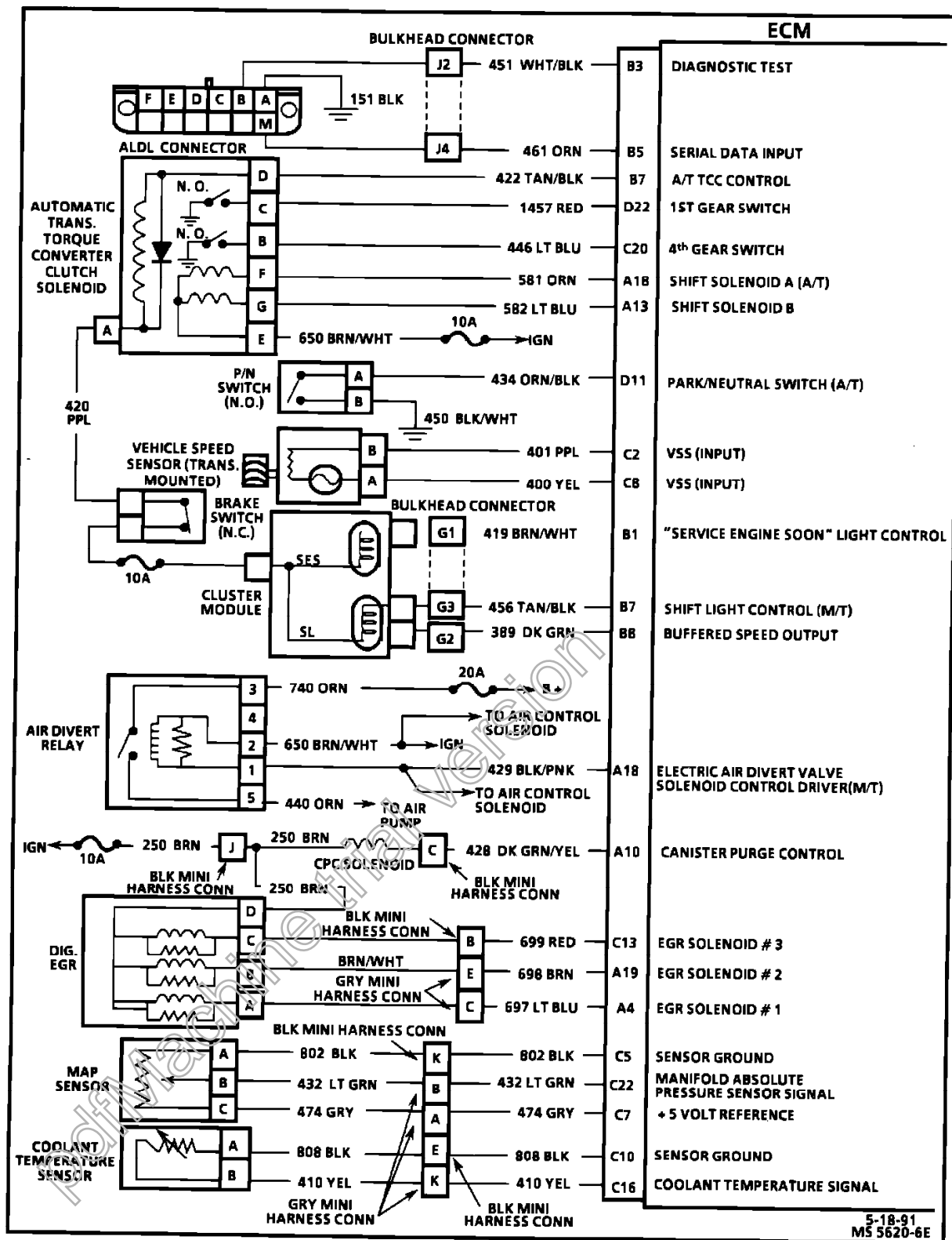
Engine Management Wiring Diagram (1 Of 3)
