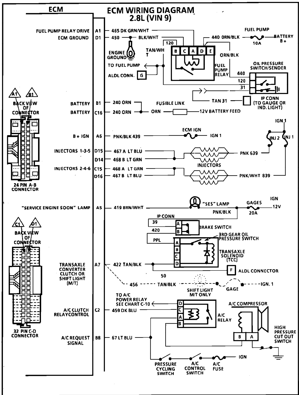
ECM Wiring Diagram (Part 2 of 2)
