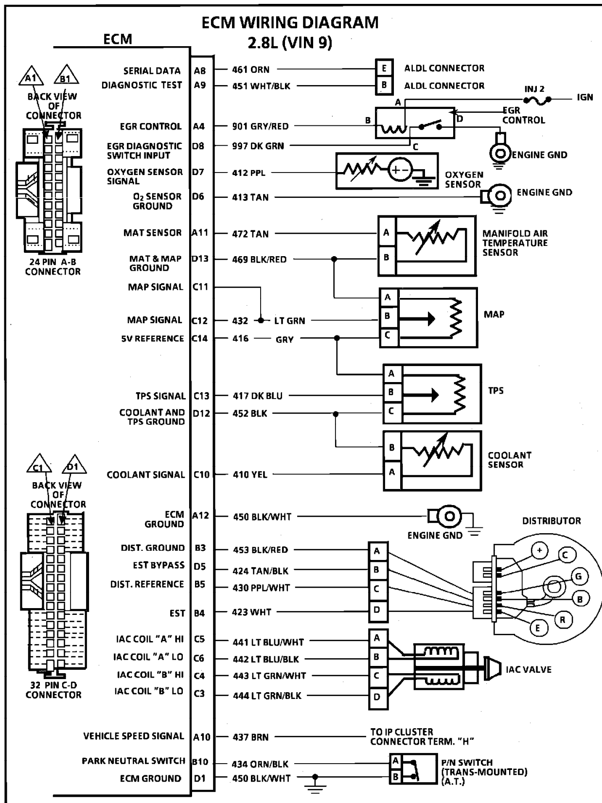
ECM Wiring Diagram (Part 1 of 2)
